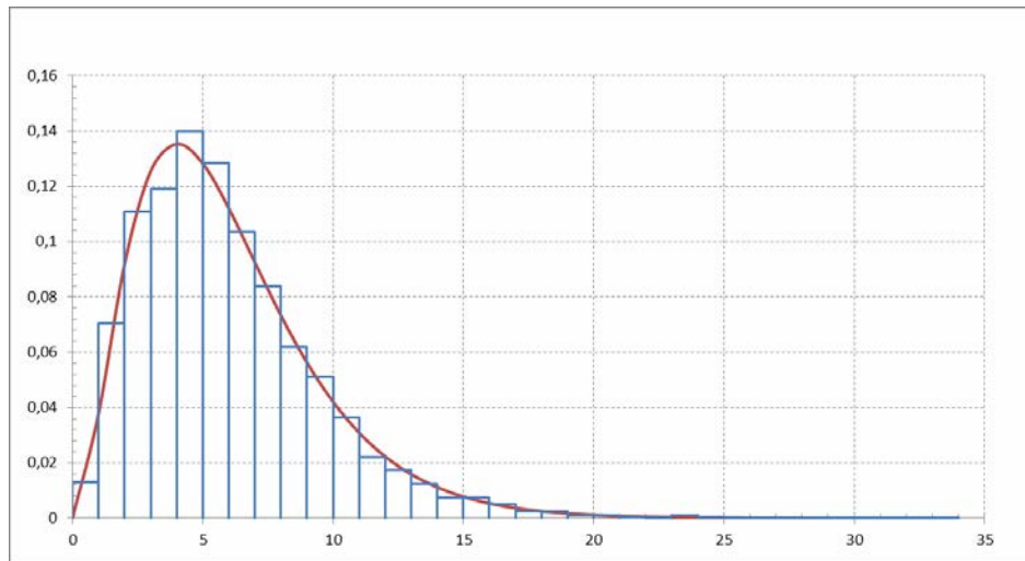
Fig. 23 Histogram for 2000 simulated interviews of 600 people compared to density for \chi^2 - distribution with (3-1)(4-1) = 6 degrees of freedom. The data are produced in column BN in Fig. 16.
