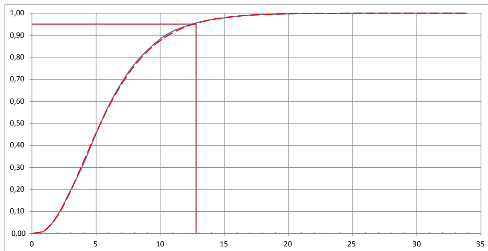
Fig. 24 Cumulated relative frequencies from Fig. 23 compared to \chi^2 - distribution with 6 degrees of freedom.
